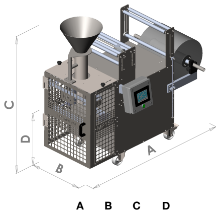
MP 150 1.165 680 998 413 mm
